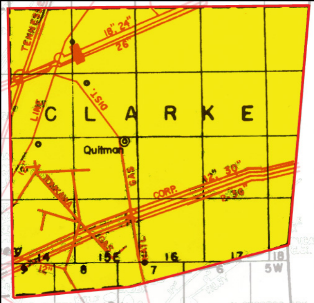
Clarke County Gas Transmission Map
